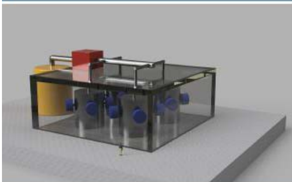
Staged Z-Pinch
